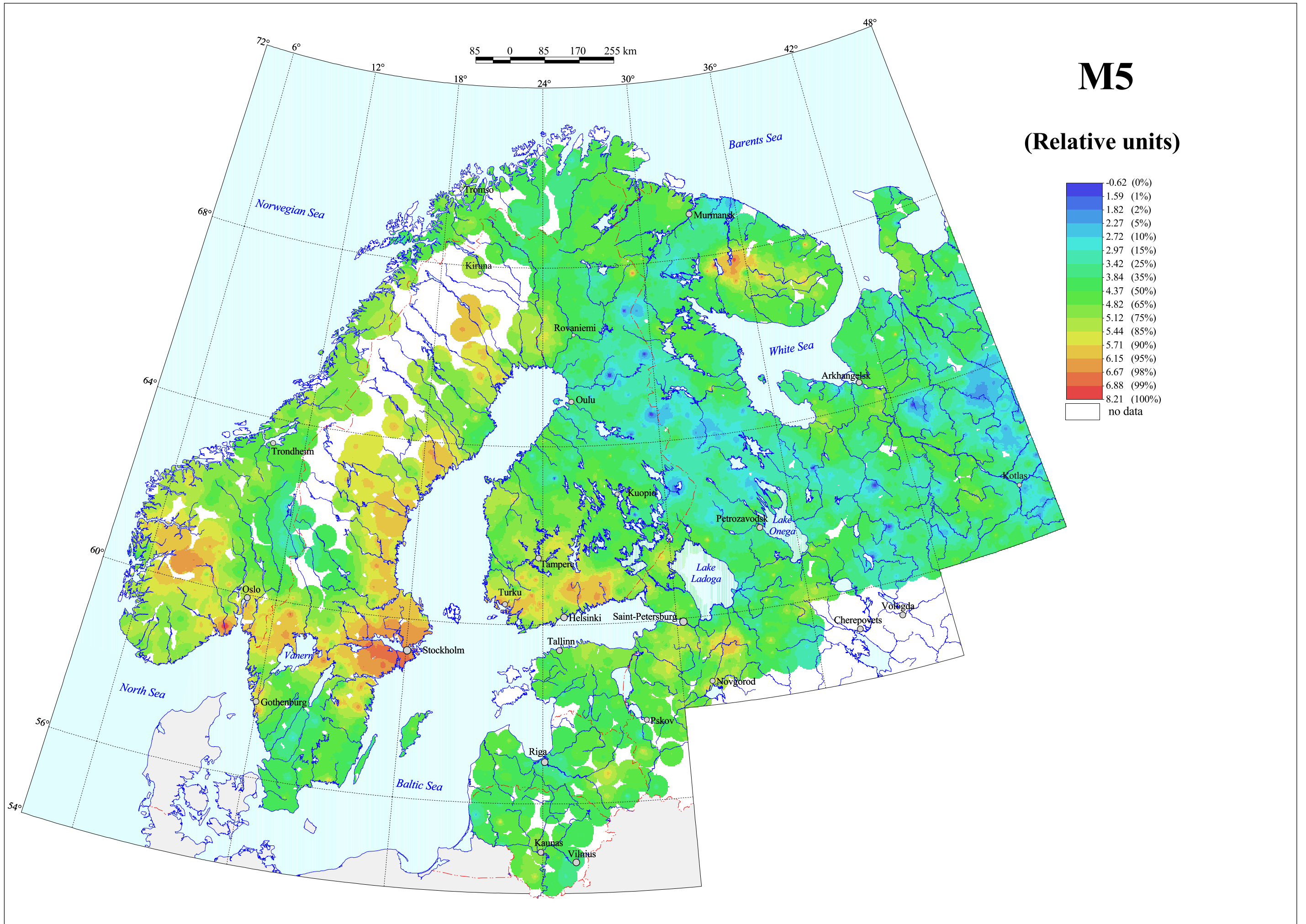
M5 (Ce, La, Sn, U, Y) in C-horizon, Grain Size <2 mm, Total Content
